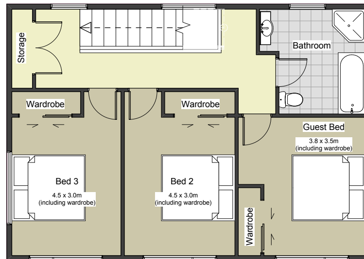
First Floor Plan 69m 2
